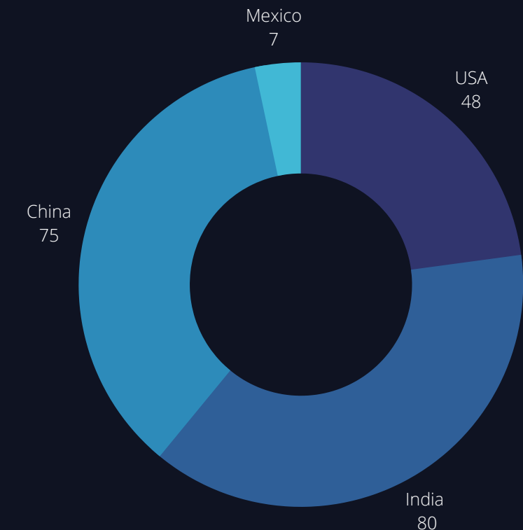
Ocean pollution of unprocessed plastic, world statistic (mln.tonns)
