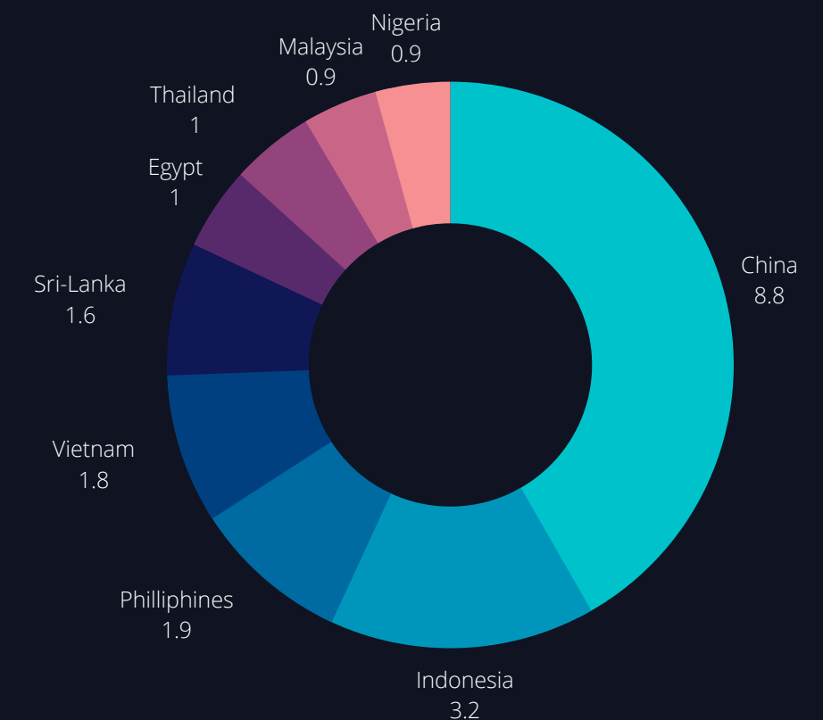
Ocean pollution of unprocessed plastic, world statistic (mln.tonns)
