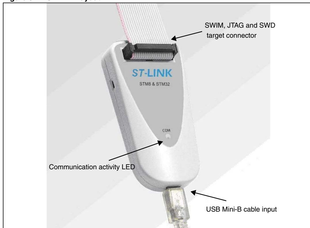
Figure 3. ST-LINK layout
